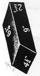
END SKEW 9" - 6 3/4" x 4 1/2" x 2 1/2" Also 60° END SKEW 9" - 7 7/8" x 4 1/2" x 2 1/2"
