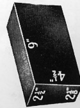
No. 1 ARCH 9" x 4 1/2" x (2 1/2" - 2 1/6")
